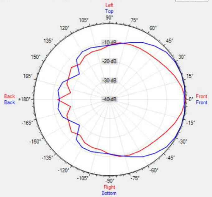
Data Shown: KUBO5T (Apart Audio) Display Parameters: Frequency: 2000Hz (1/24th Octave)
