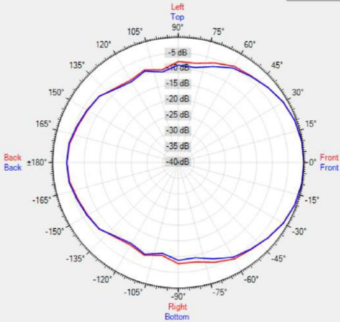
Data Shown: KUBO5T (Apart Audio) Display Parameters: Frequency: 1000Hz (1/24th Octave)
