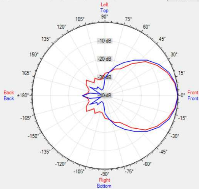
Data Shown: KUBO5T (Apart Audio) Display Parameters: Frequency: 4000Hz (1/24th Octave)
