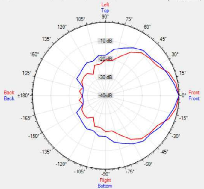
Data Shown: KUBO5T (Apart Audio) Display Parameters: Frequency: 8000Hz (1/24th Octave)
